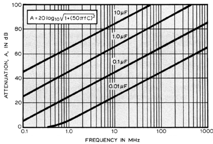
ATTENUATION CHARACTERISTICS FOR IDEAL CAPACITORS AT 50 Ω IMPEDANCE, PER MIL-STD-220
